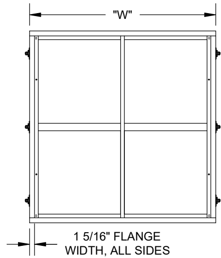
FLANGE CONNECTION
